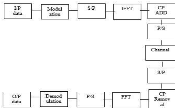
Fig. 1 OFDM Transceiver\
